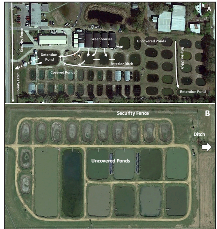
Figure 2. Farm layout figure for (A) ornamental fish production in Florida (University of Florida Tropical Aquaculture Laboratory) and (B) catfish production in Mississippi (Thad Cochran National Warmwater Aquaculture Center fish-health ponds). (A) There are at least 3 CCPs for the ornamental fish facility, including movement of water from greenhouse to interior ditch and ponds, from the interior ditch/pond complex to the detention pond, and from the detention pond to the county ditch. The most important CCP is the connection between detention pond and ditch. (B) The catfish fish-health research facility has only a single location for effluent; this would be a major CCP. Facilities vary in configuration of ponds, ditches, and buildings and in the movement of effluent offsite. While both industries rely on outdoor production ponds, their hazards and ultimately CCPs differ.
