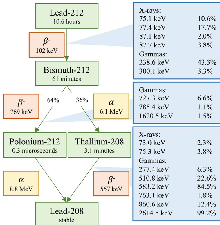
Fig. 1 Decay scheme of ^{212}\text{Pb} . The mean alpha and beta energies are included. The relevant photons emitted and their energies are added to the transition. Photons with emission probabilities smaller than 1% per ^{212}\text{Pb} decay or with energies below 70 keV are not included. The data are taken from ICRP 107 [18]
